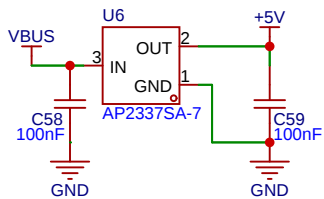
USB Inrush Limiter
