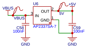
USB Inrush Limiter
